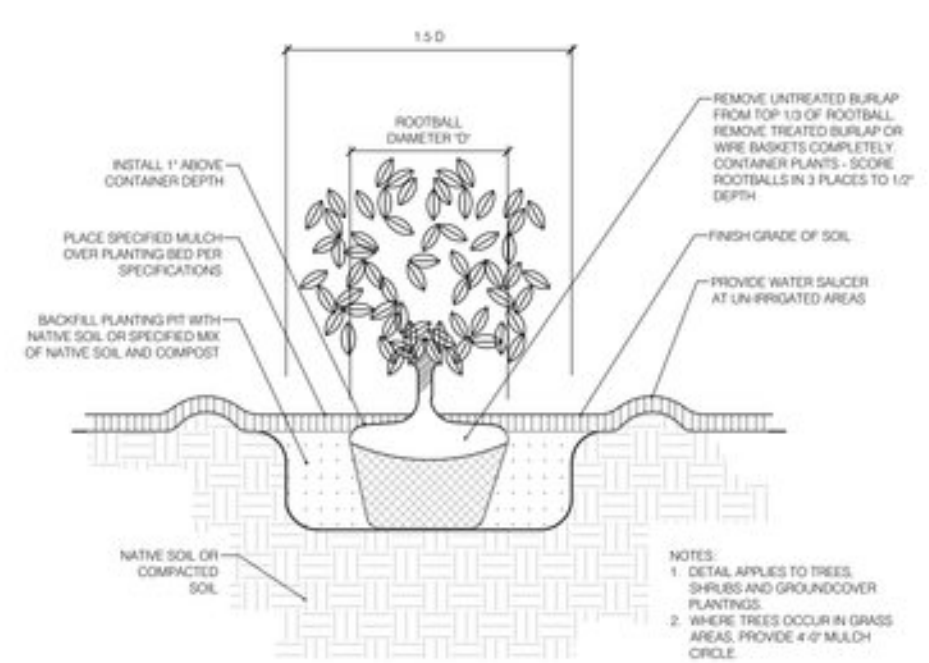
1 TYPICAL TREE AND SHRUB PLANTING SCALE: NTS
