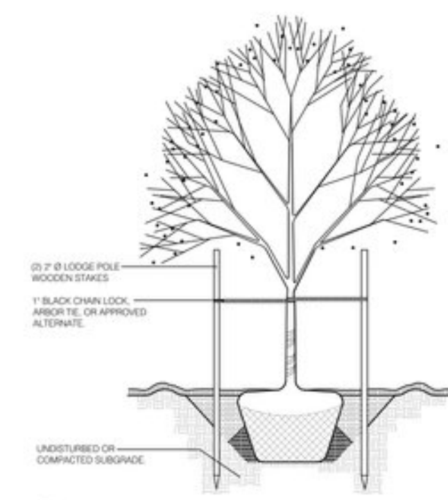
5 TYPICAL TREE STAKING SCALE: NTS
