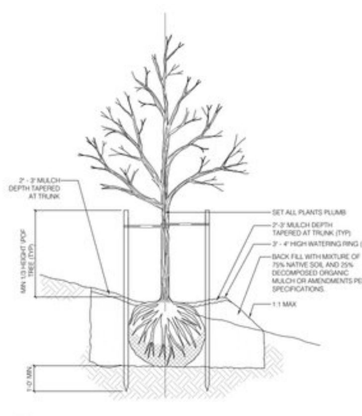
3 TYPICAL TREE PLANTING ON SLOPE SCALE: NTS
